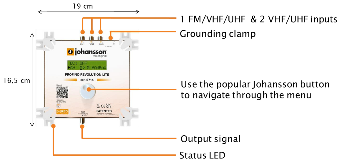
FIGURE 1: TOP VIEW OF PRODUCT
